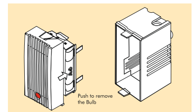
Details showing assembly replacement of Bulb/Glass tube Fuse.
