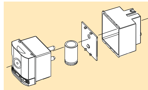
Exploded view of assembly
